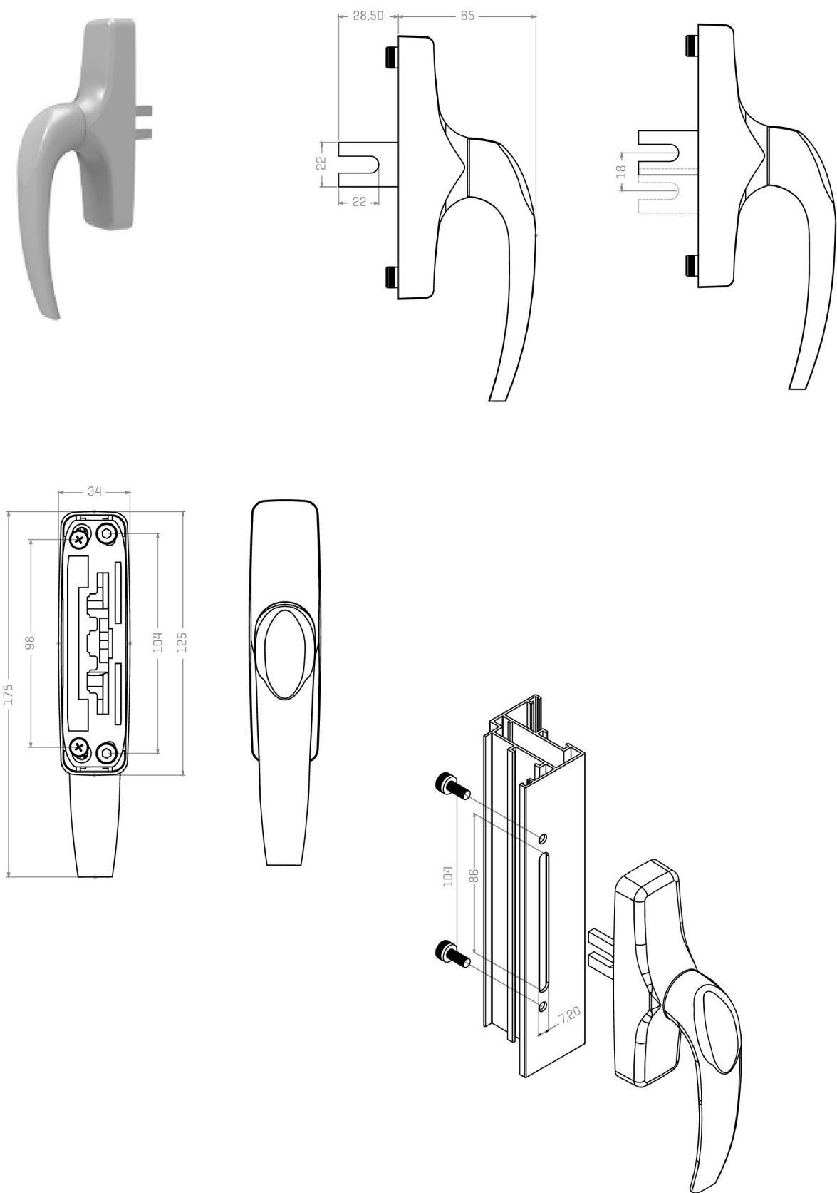
Finger Print Cremone Bolt (Single Fork)
